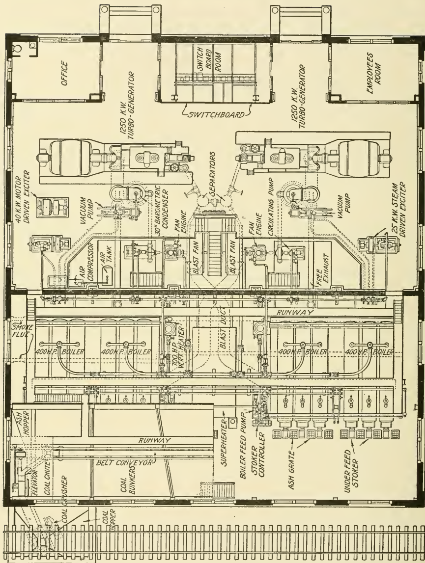
Fig. 149. Plan of St. Clair Tunnel Power Plant of the Grand Trunk Railroad
